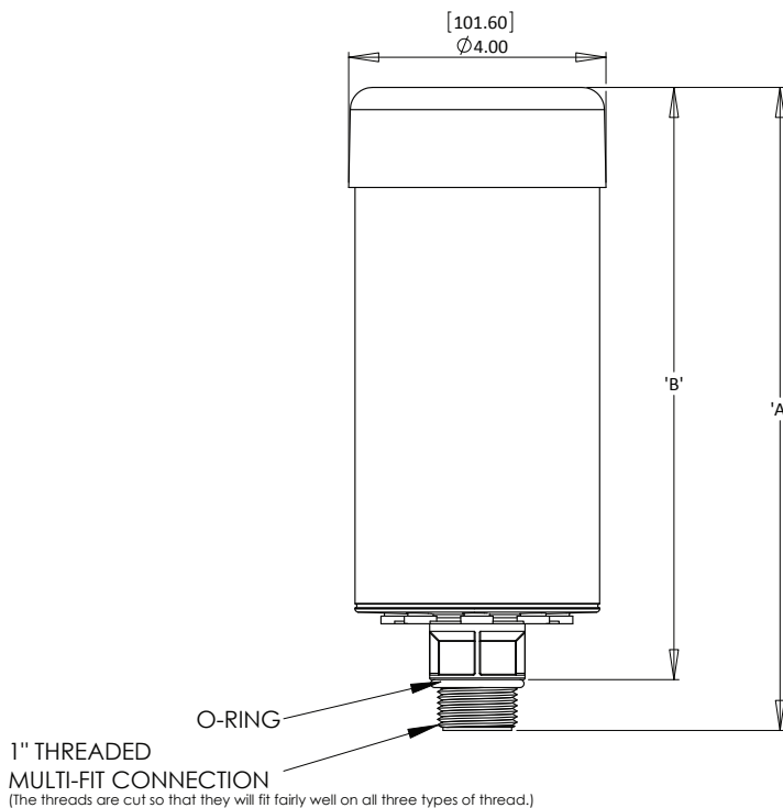
Field Adapter
